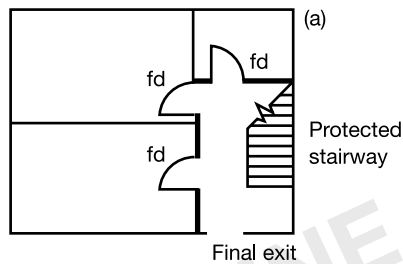
Diagram 2 Alternative arrangements for final exits
