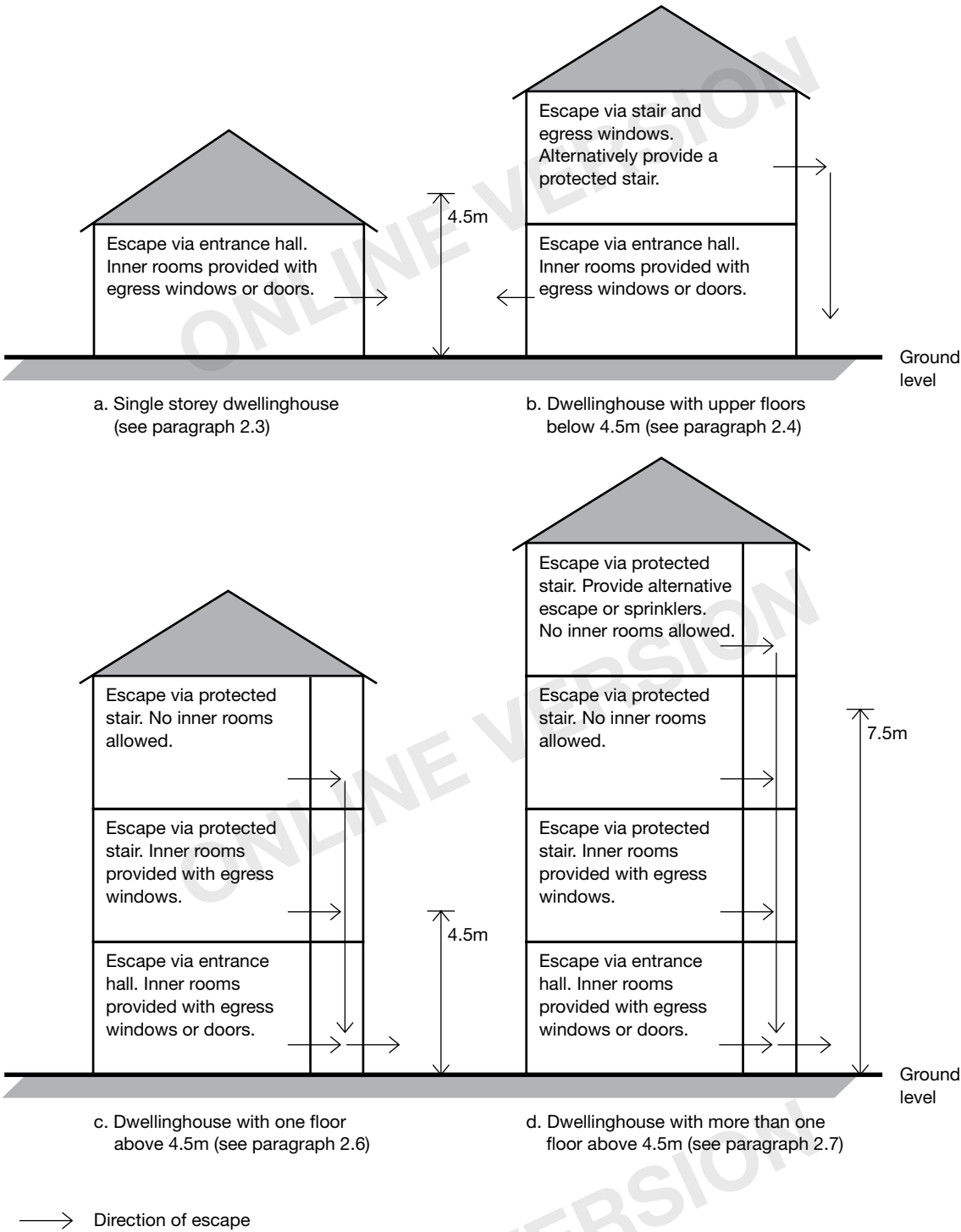
Diagram 1 Means of escape from dwellinghouses
