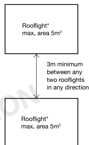
Diagram 23 Limitations on spacing and size of plastic rooflights having a Class 3 (National class) or Class D-s3, d2 (European class) or TP(b) lower surface
